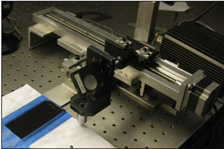
Figure 2. Original linear translation system with focusing optics.
