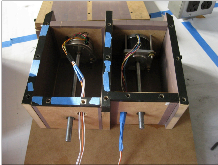
Figure 9. Feed (left) and print (right) piston prototype.
