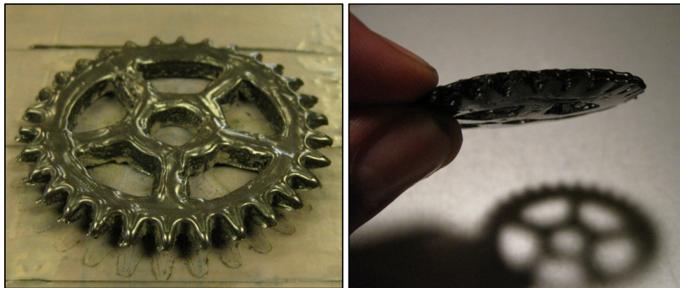
Figure 10. A printed gear, left, and thermal warping of a printed gear, right. The ends of the spurs are significantly less thick than the base.
