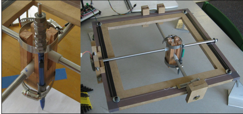
Figure 7. Early version of the translation head, showing the reamed nylon bushings mounted in a block of wood (left) and an overview of the complete translation system (right).
