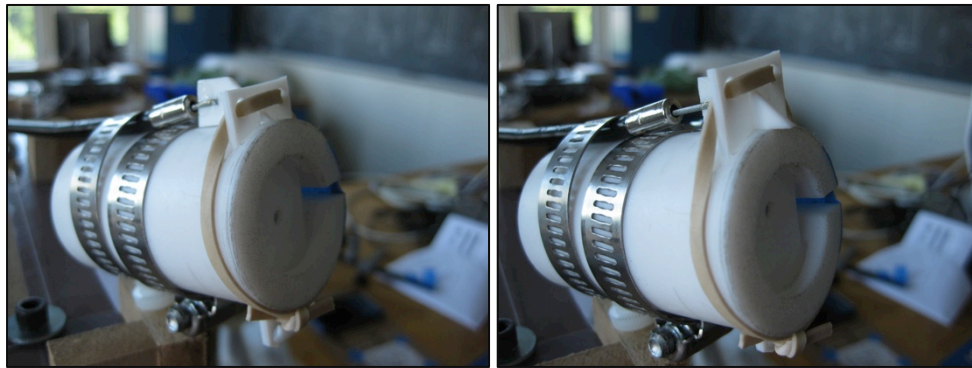
Figure 16. The revised shutter open (left) and closed (right).
