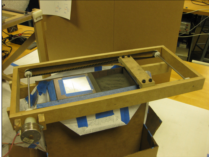
Figure 12. The fourth, and moderately successful powder distribution mechanism.
