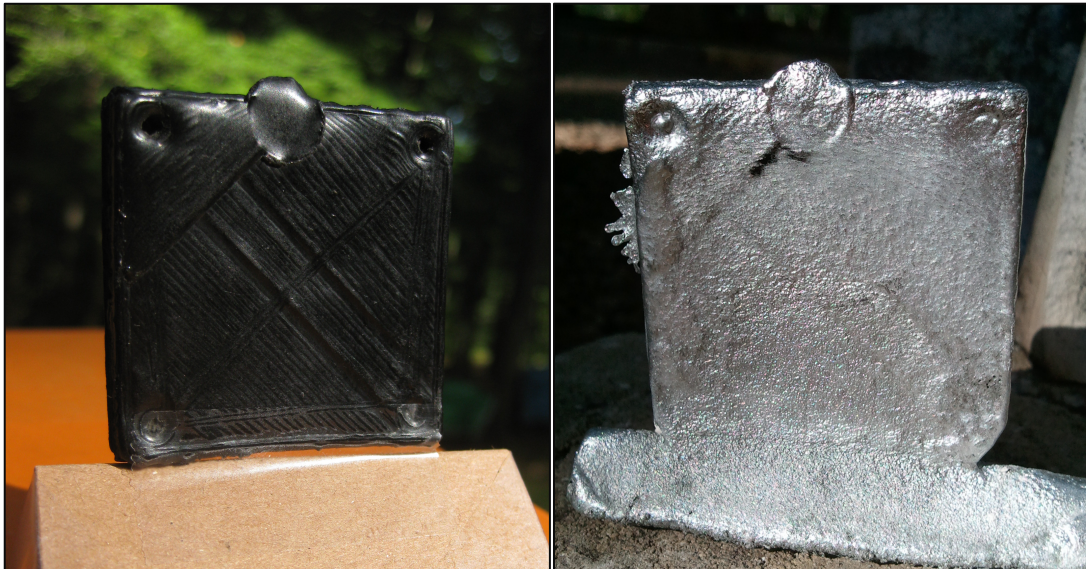
Figure 19. Result of lost wax casting of a printed test block.
