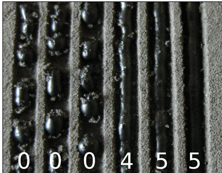
Figure 4. Candelilla wax sinter test results. The two beads on the right were assigned sinter indices of five. The three on the left were assigned sinter indices of zero.
