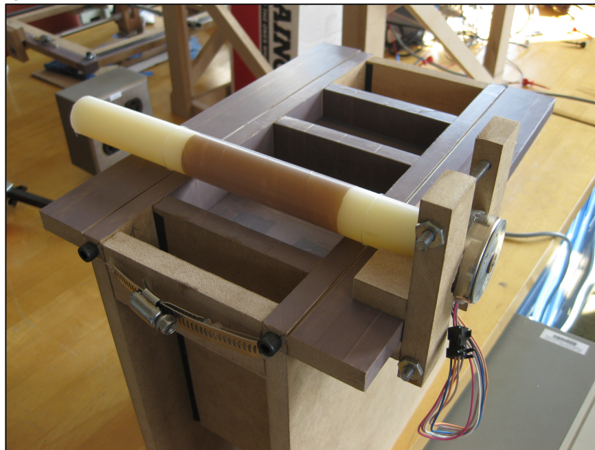
Figure 11. The first, failed powder distribution mechanism.
