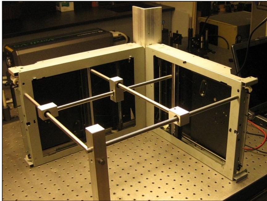
Figure 6. The first prototype 2D translator was made from two salvaged flatbed scanners.
