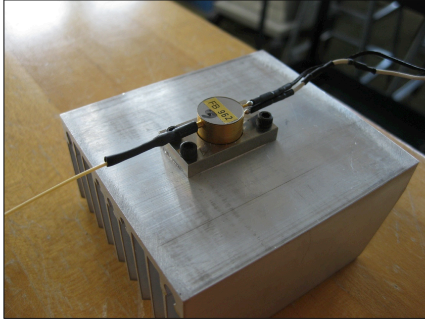
Figure 13. Laser diode affixed to heat sink. The diode is powered by the lines on the right and emits into the fiber optic cable seen at left.
