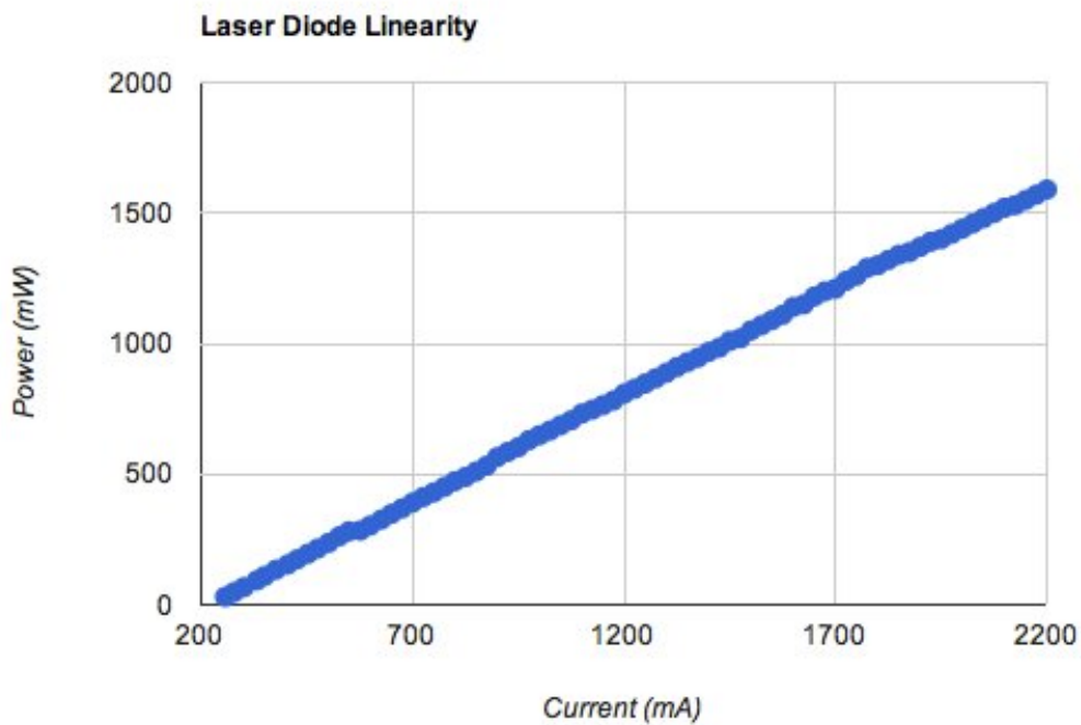
Figure 14. The laser diode behaves predictably linearly up unto 2.2 Amps, where power output begins to decrease.
