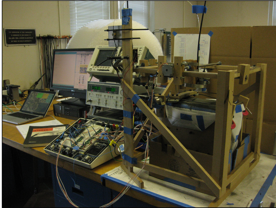
Figure 23. The 3D printer prototype in action.
