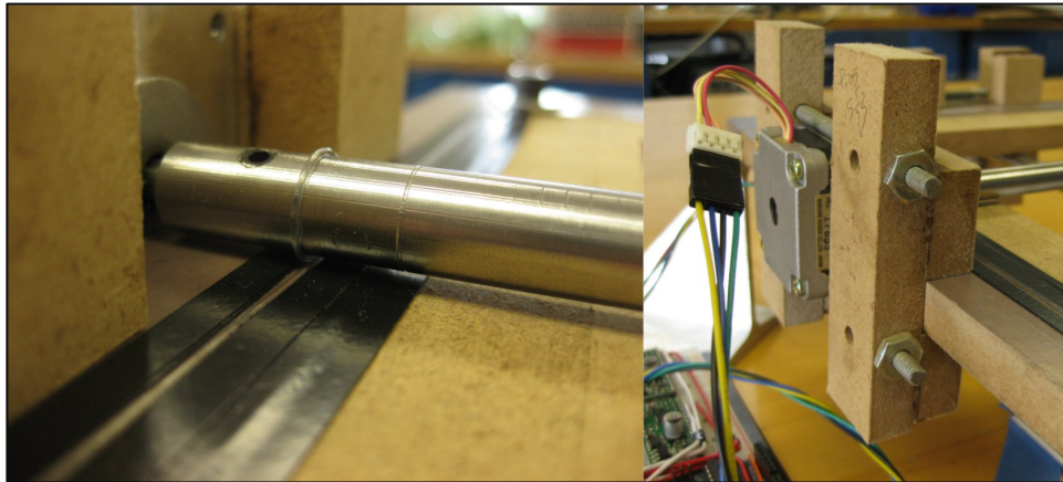
Figure 8. Detail of the cable-wrapping of the gantry rod (left) and one of the two motor mounts used in the translation system (right).
