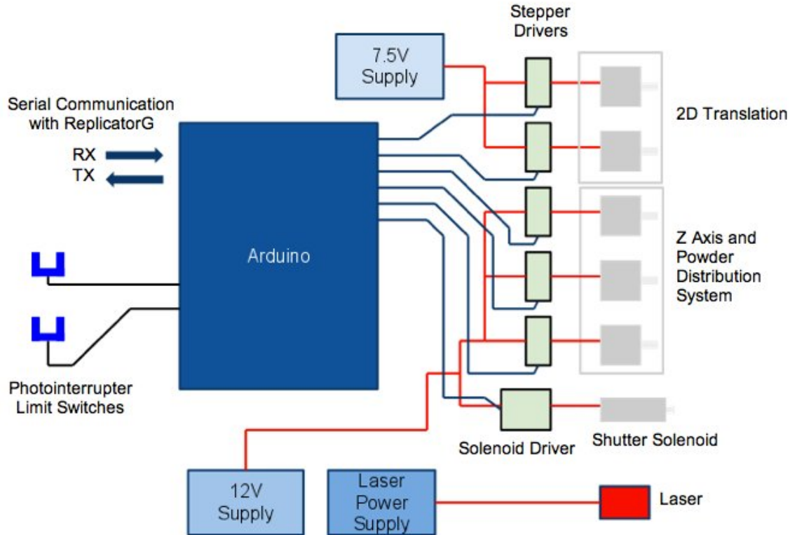
Figure 17. Diagram of the electronics that run the device.
